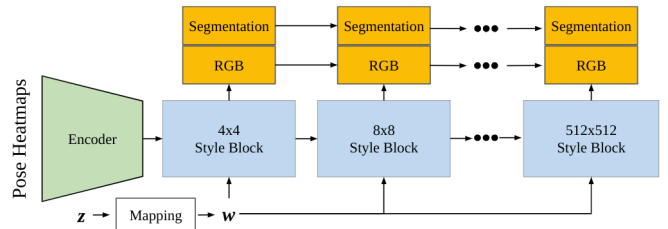
Figure 3: We trained a pose conditioned StyleGAN2 network, that outputs both an RGB image as well as a segmentation of the image in each layer. Pose heatmaps are encoded and inputted into the first style block in StyleGAN2 instead of a constant input.
