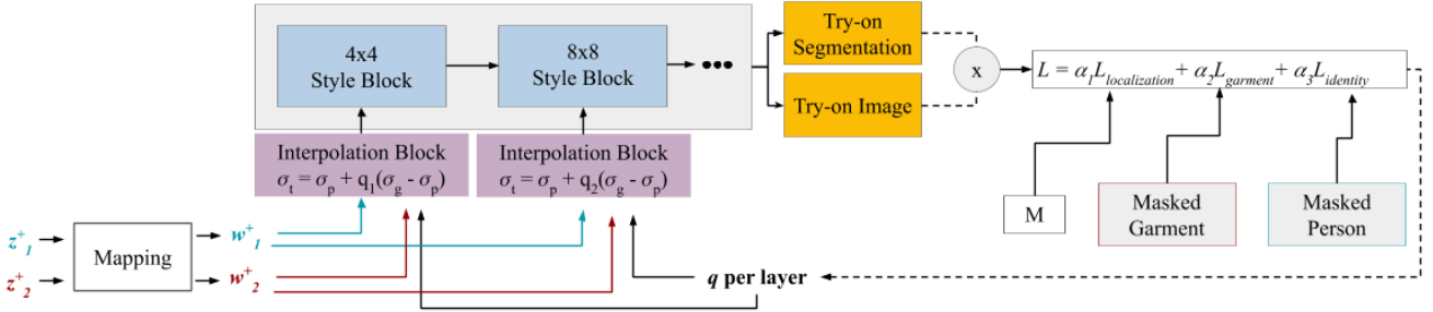
Figure 2: The try-on optimization setup illustrated here takes two latent codes z_1^+ and z_2^+ (representing two input images) and a pose heatmap as input into a pose-conditioned StyleGAN2 generator (gray). The generator produces the try-on image and its corresponding segmentation by interpolating between the latent codes using the interpolation-coefficients q . By minimizing the loss function over the space of interpolation coefficients, we are able to transfer garment(s) g from a garment image I_g , to the person image I_p .
